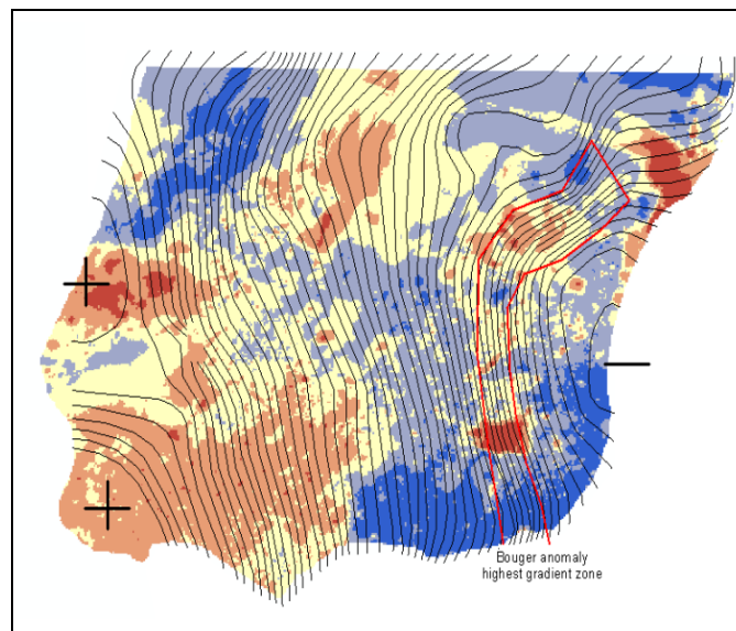
Figure 4: Kriged PSI data compared to 1st degree Bouguer anomaly contours. +/- indicate positive/negative anomalies. The red line depicts the area of smallest contour spatial separation, or strongest gravimetric gradient.
