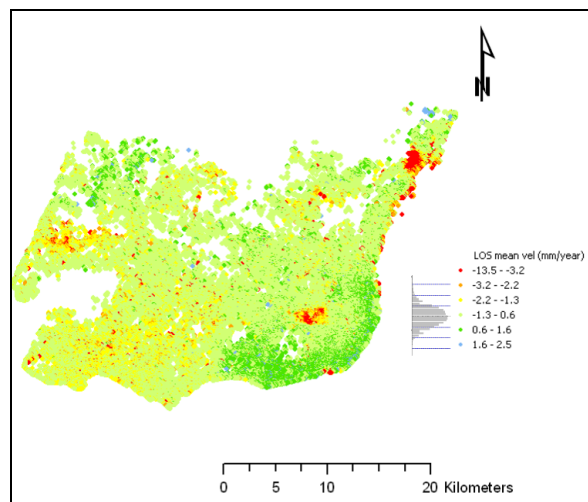
Figure 2: Altamira's psi mean velocity map
