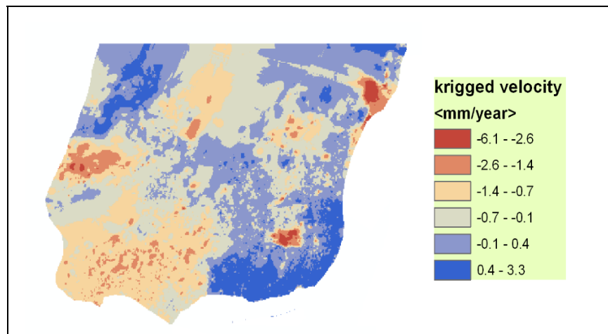
Figure 3: Kriged PSI data
