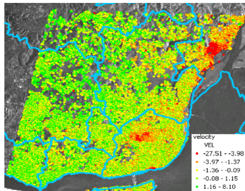
Figure1: TRE's psi mean velocity map (in mm/yr)
