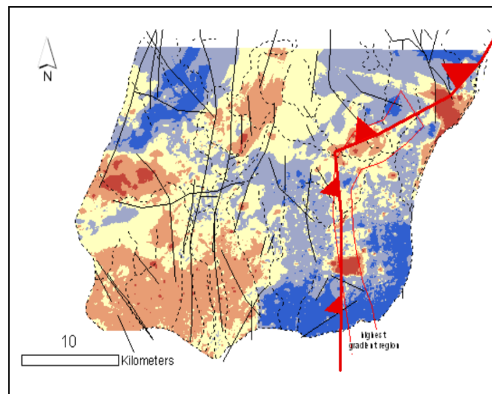
Figure 5: Comparison of kriged PSI data with outcropping faults (black solid lines), drainage network (black dotted lines), and independently-interpreted fault zone (red line with filled triangles) by Carvalho et al. (2007).
